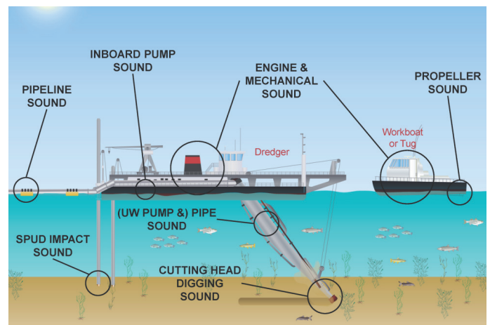
Figure 1 Schematic overview of a cutter suction dredger
